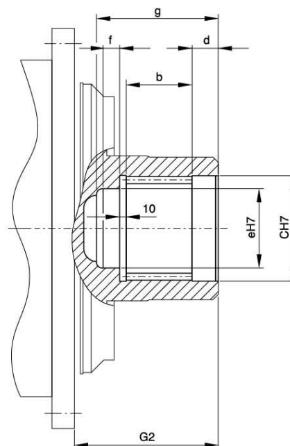
花键齿形按 DIN 5480 Hollow shaft with involute splines acc. to DIN 5480.
