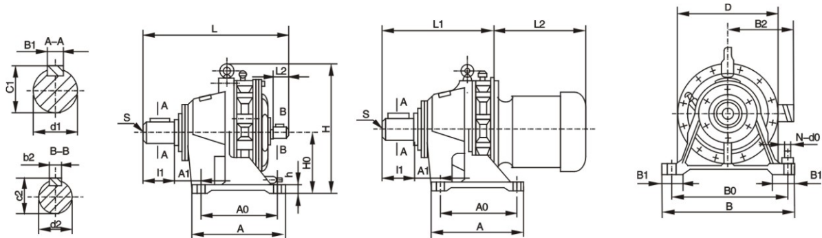
XW(D)型卧式单级外形安装及联接尺寸 XW(D) type. (Horizontal Single stage) overall and mounting dimensions
